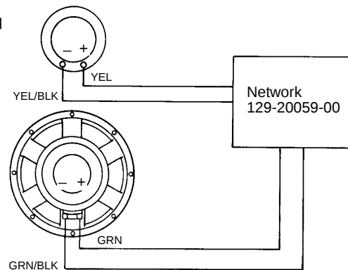
SCHEMATIC (129-20059-00)
