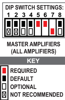
Figure 5.20 – DIP Switch Settings for Parallel Configuration
